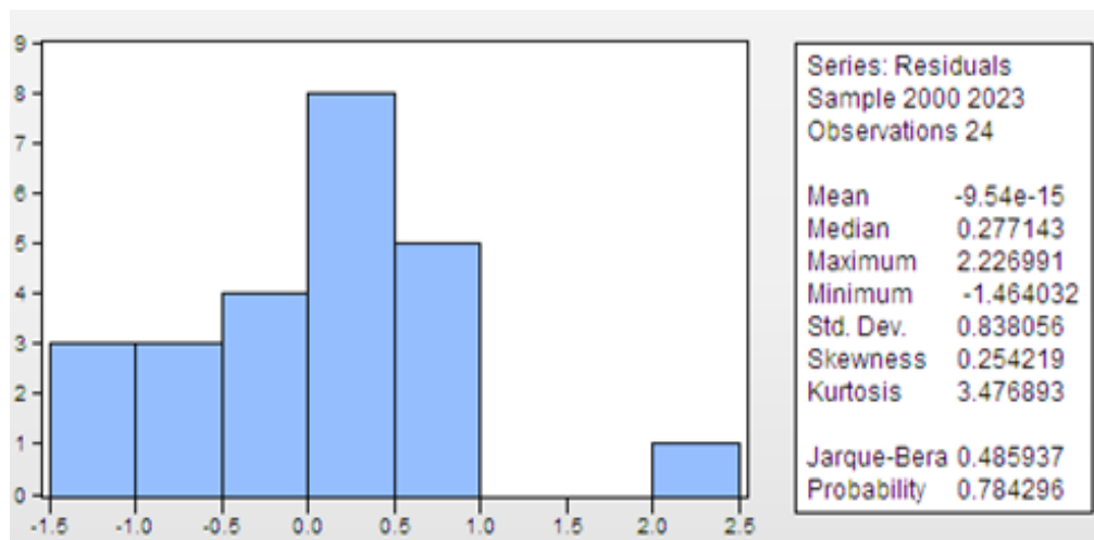
Figure (01): Results of the Jarque-Bera Test
